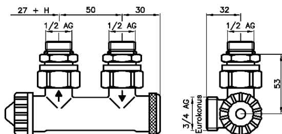
Vario THK M, angled – version G \frac{1}{2} male thread
