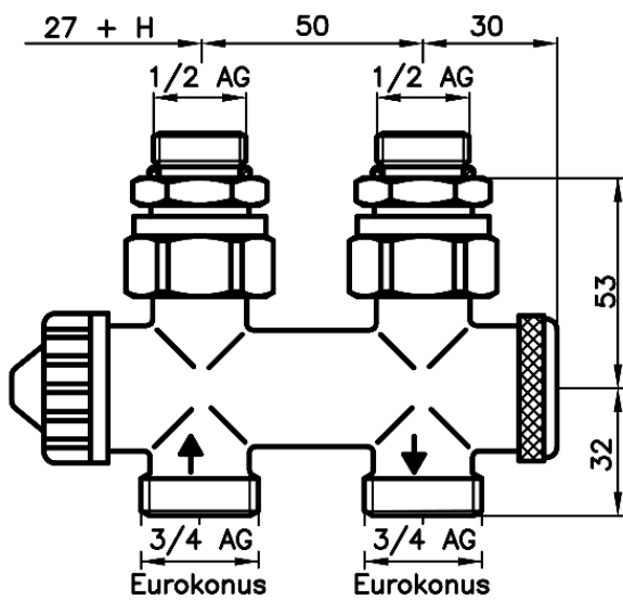
Vario THK M, straight – version G½ male thread
