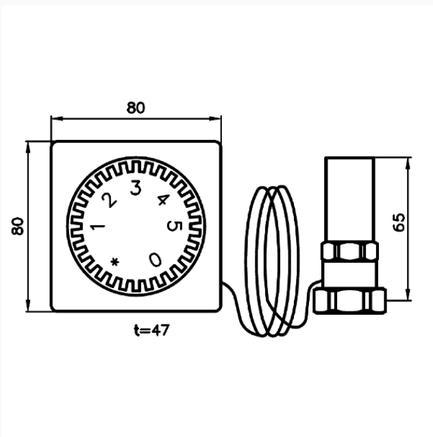
Dimensions (mm)
