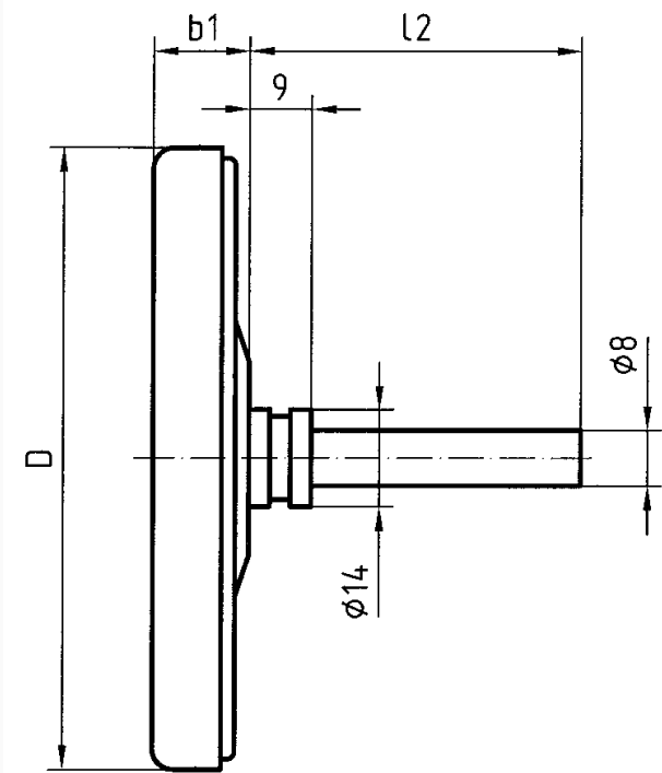
centre back connection, plain
