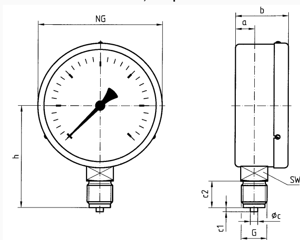
NG 160 – bottom connection, with push on bezel
