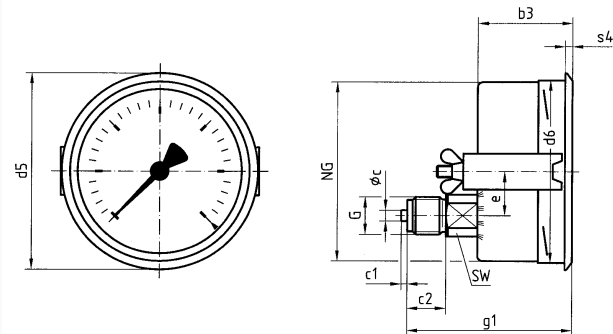
Dimensions (mm)
