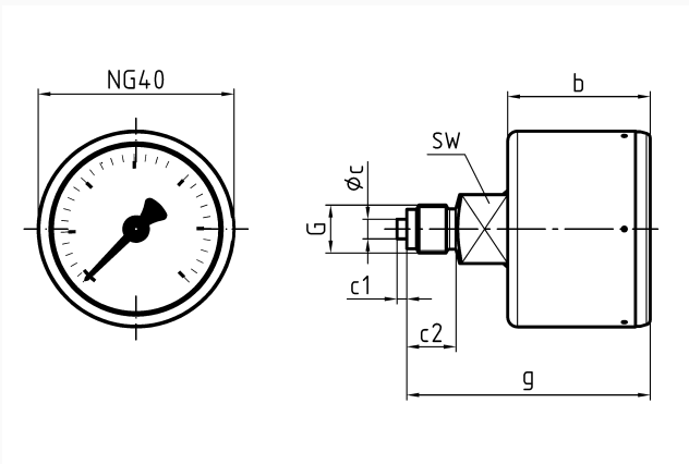
Dimensions (mm)
