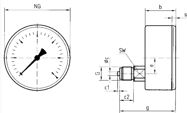
Dimensions (mm)
