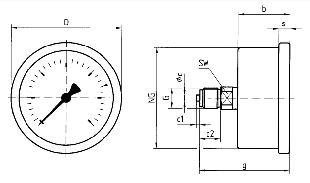
Dimensions (mm)
