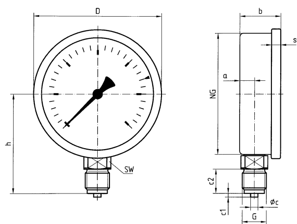
Dimensions (mm)
