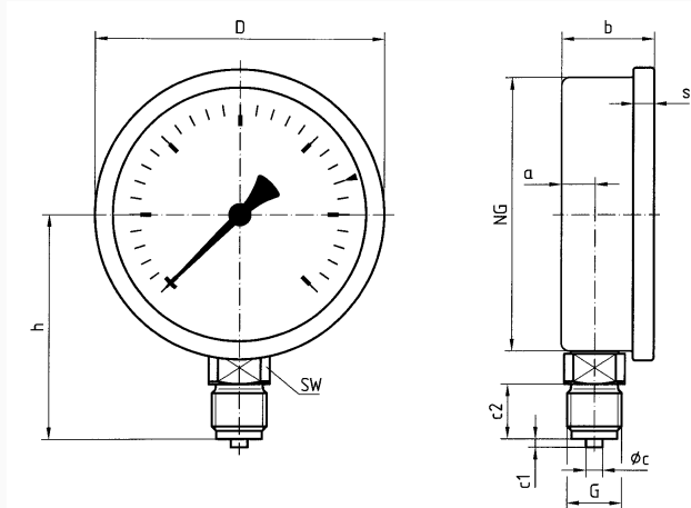
Dimensions (mm)
