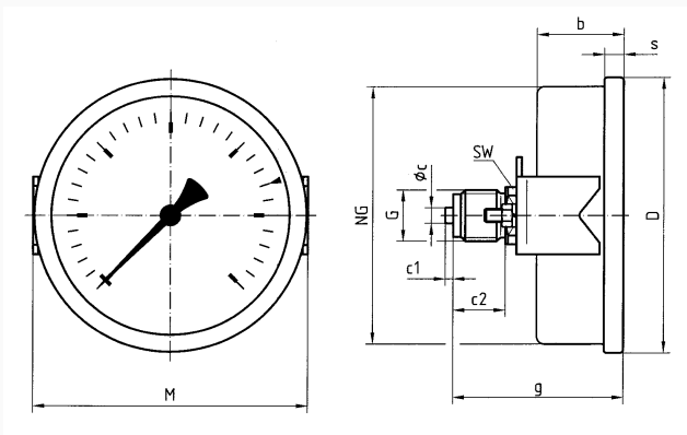
NG 100 – centre back connection, with clamp fixing
